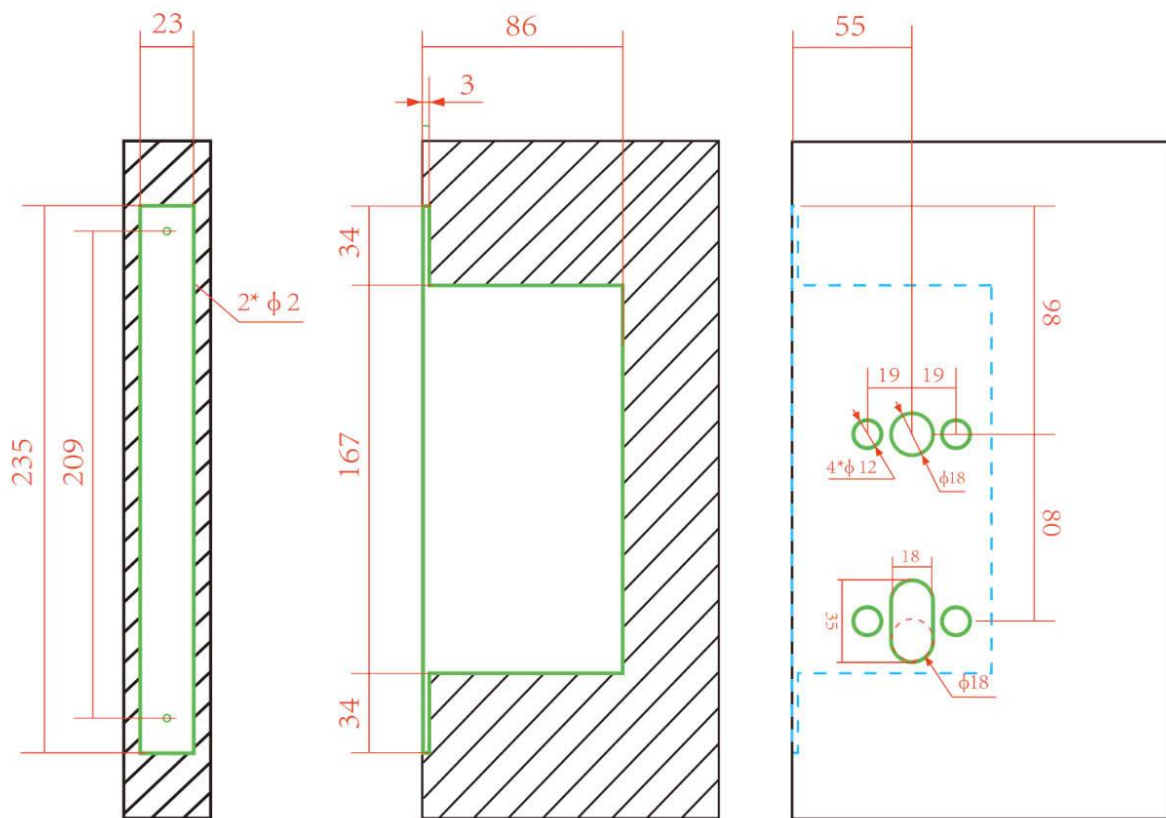
K5572 /Opening size drawing
